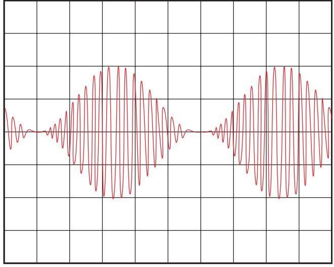
The picture shows: internal source, V_o = 10 V_{pp} , f = 20 \text{ kHz} , 100 % modulation, scope 5 V/cm.
